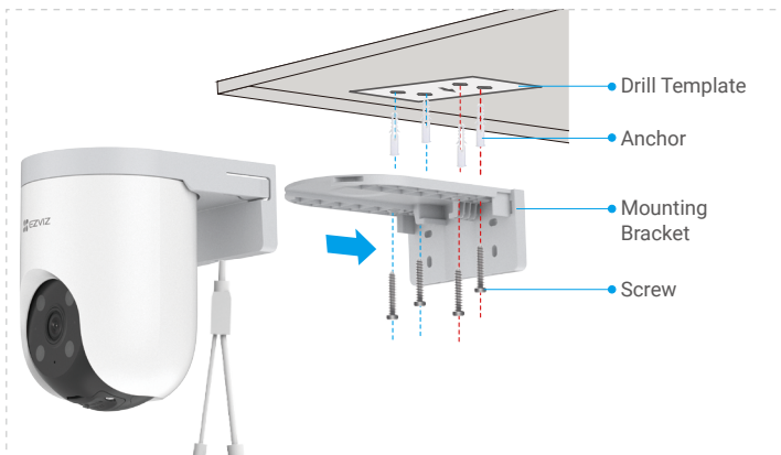
Fig. 1 Ceiling Mount
